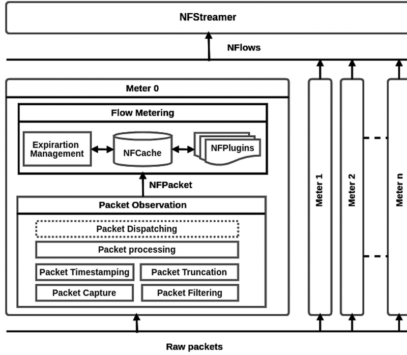
Fig. 1. NFStream overall architecture.
