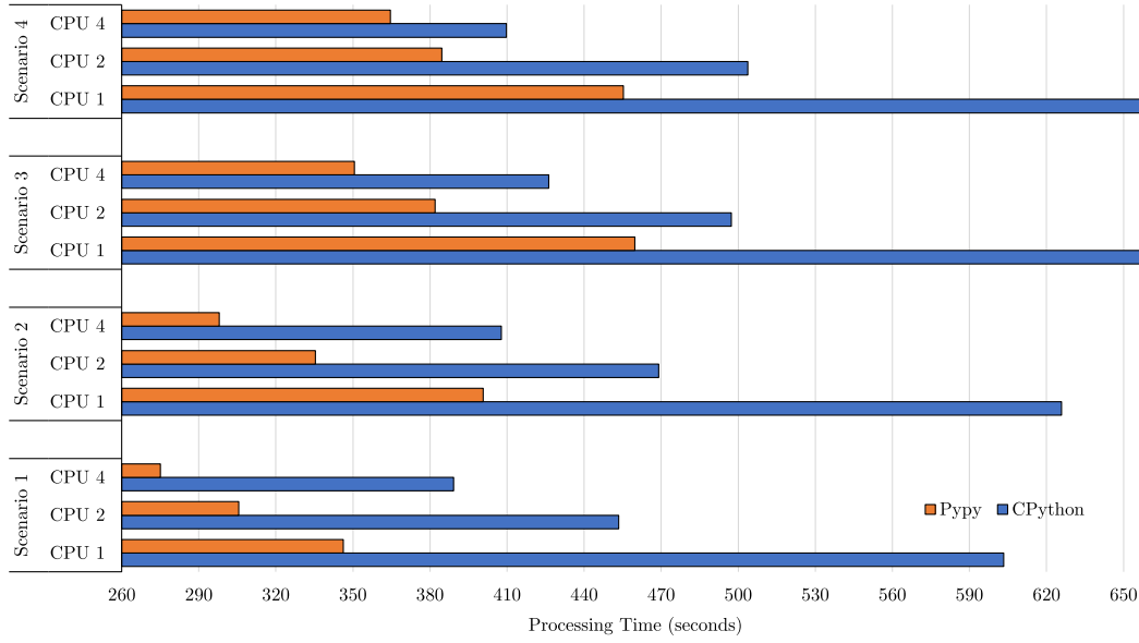
Fig. 2. CPython vs. PyPy NFStream processing times relative to the number of used cores.
